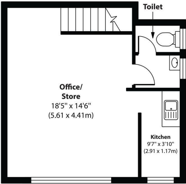
First Floor Approximate Floor Area 346 sq. ft (32.10 sq. m)
